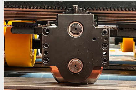
HORIZONTAL CUTTING
