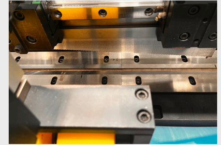
HORIZONTAL SLOTTING & SCORING
